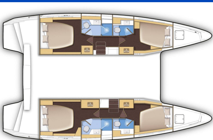
Version 4 cabins / 4 cabin version
