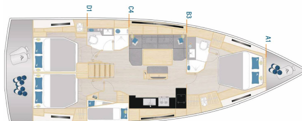
460 OPTION INTERIOR LAYOUT
